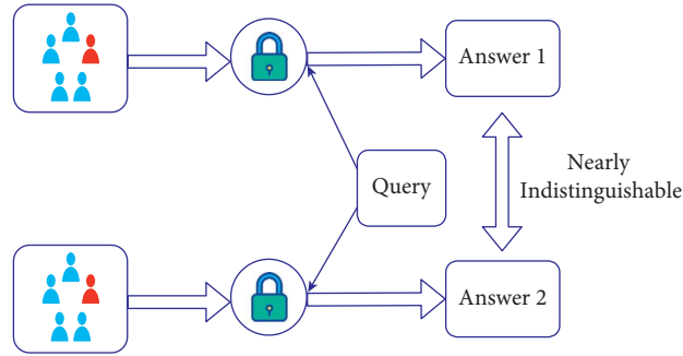
FIGURE 1: Differential privacy.
