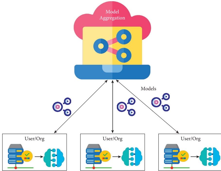
FIGURE 5: FL architecture.
